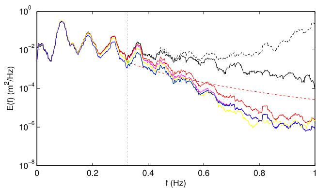
Fig. 7. Surface elevation energy density spectra E(f) . AST measurements: \zeta_m (black line); hydrostatic reconstruction: \zeta_H^{\delta m} (blue line); TFM - sharp cutoff: \zeta_{L,SH} (green line); TFM - linear cutoff: \zeta_{L,L} (magenta line); TFM - steady cutoff: \zeta_{L,ST} (red line); TFM - Jonswap: \zeta_{L,J} (red dashed line); TFM - no cutoff \zeta_{L,NC} (black dashed line); semi-empirical TFM: \zeta_N (yellow line); see the associated equations in Table 1 f_c = 0.32 Hz (vertical black dotted line). The spectra have been averaged over 1/66 Hz. (For interpretation of the references to color in this figure legend, the reader is referred to the Web version of this article.)
