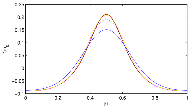
Fig. 4. Surface elevation of a periodic weakly nonlinear wave, \varepsilon = 0.15 , \mu = 0.25 , \delta_m = 0 . Full Euler solution (black line); hydrostatic reconstruction: \zeta_H^{\delta_m} (blue line); linear formula in space: \zeta_{L,space} (magenta dashed line); fully-dispersive nonlinear reconstruction in space: \zeta_{NL,space} (red line); heuristic reconstruction in space: \zeta_{HE,space} (yellow line); see the associated equations in Tables 1 and 2 (For interpretation of the references to color in this figure legend, the reader is referred to the Web version of this article.)
