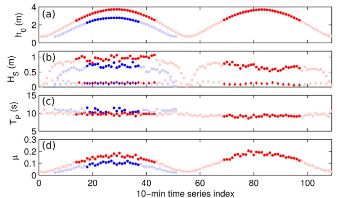
Fig. 6. Wave and tide conditions for both experiments (LS1 in blue and LS2 in red). (a) Mean water depth h_0 ; (b) Short-wave significant wave height H_{s,short-wave} (circles) and infragravity significant wave height H_{s,infrac} computed over 20 min (diamonds); (c) Spectral peak period T_p ; (d) Shallowness parameter \mu . Dark-colored points and light-colored points show data outside and inside the surf zone, respectively. Transitions between both areas represent the outer surf zone limits. In the present study, we only focus on the dark-colored points. (For interpretation of the references to color in this figure legend, the reader is referred to the Web version of this article.)
