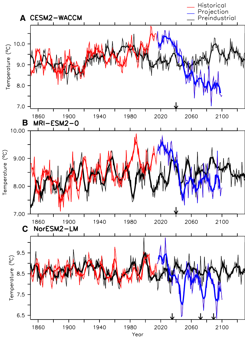
Figure 1. Examples of abrupt changes found in the subpolar gyre. Time series of surface atmospheric temperature (in °C) averaged over the SPG ( 50–10°W, 45–60°N ) in annual mean (thin line) and 5-year running mean (thick line). In black is the preindustrial simulation, in red the historical simulation, and in blue the projection considered for (A) the CESM2-WACM model with the ssp126 scenario, (B) the MRI-ESM2-0 model with the ssp245 scenario, and (C) the NorESM2-LM model with the ssp126 scenario. The black arrows represent the approximate starting of the abrupt events.
